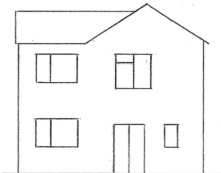
REAR ELEVATION-EXISTING. LOOKING NORTH
