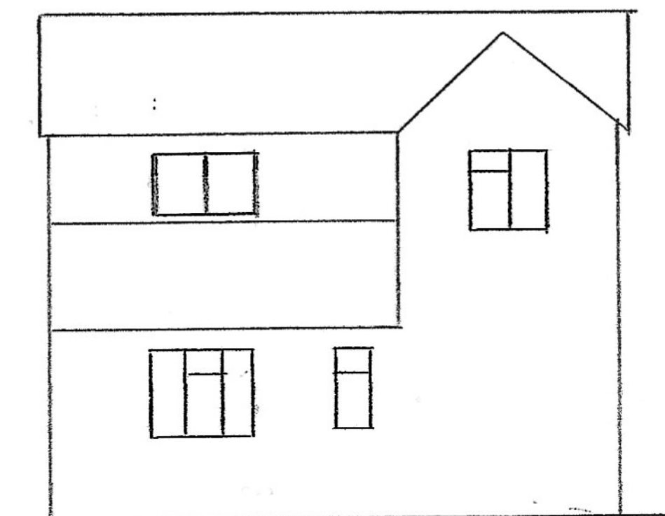
SIDE ELEVATION - PROPOSED. LOOKING EAST.
