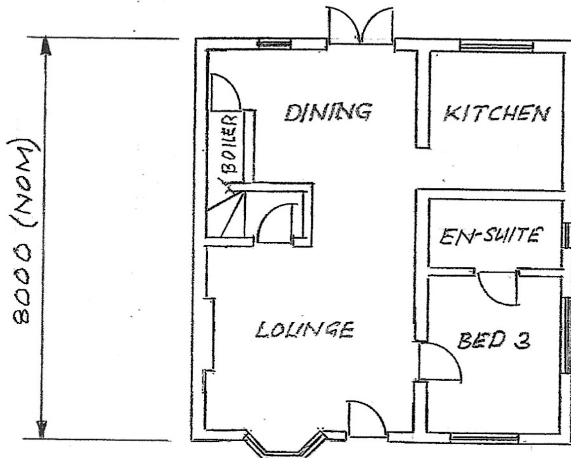
GROUND FLR PLAN - PROPOSED. LOOKING SOUTH.
