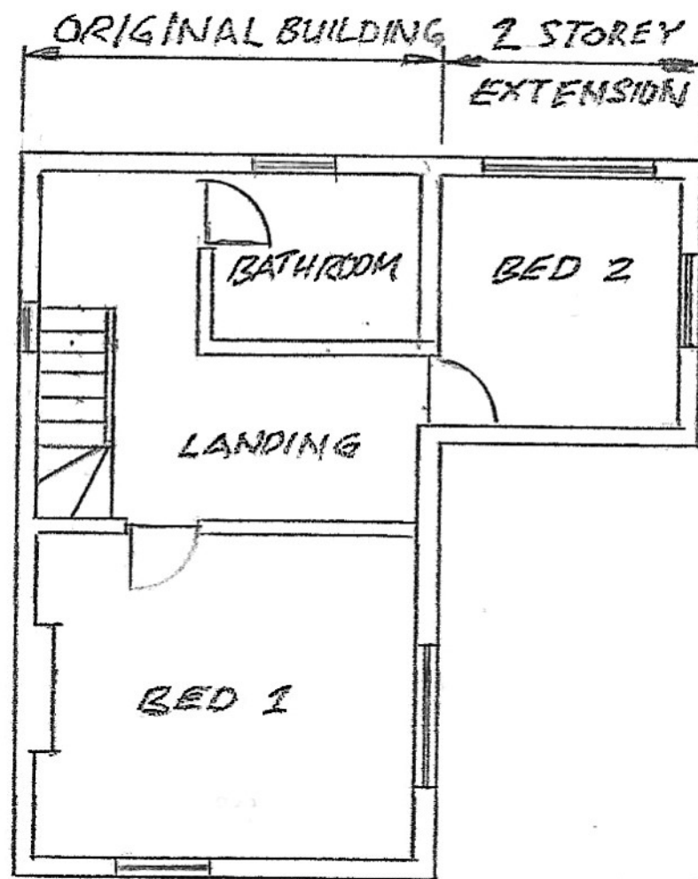
FIRST FLR PLAN - PROPOSED.
