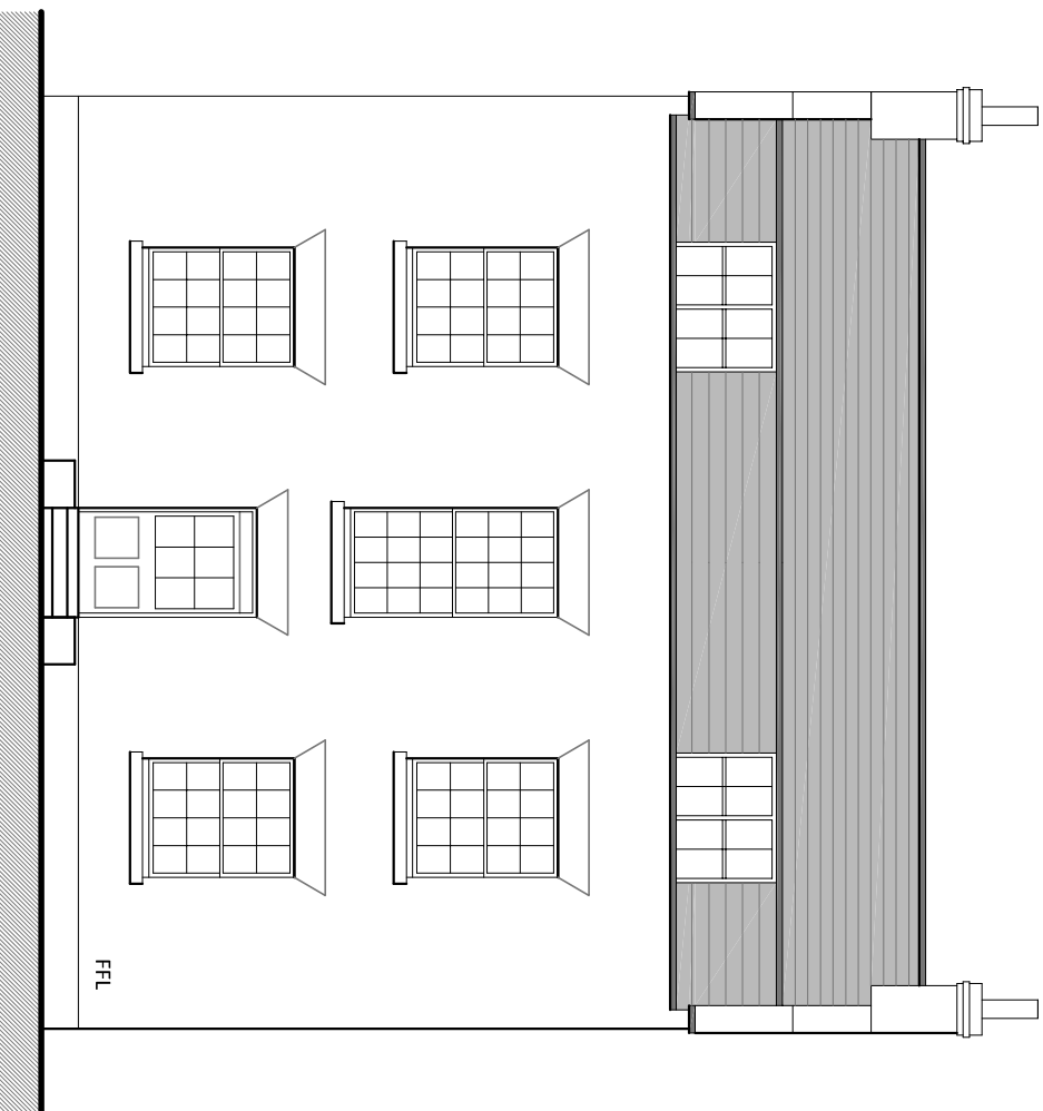
Front Elevation (West Facing)
