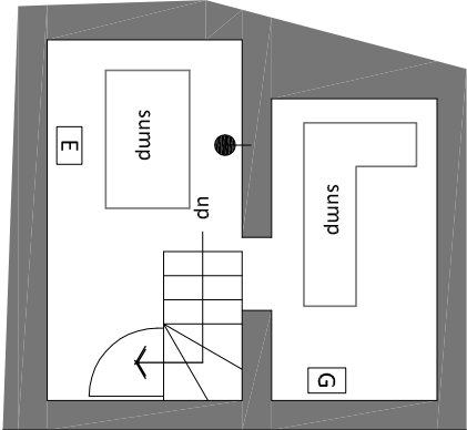
Basement Plan
