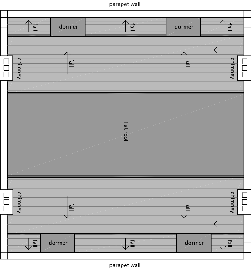
Roof Plan
