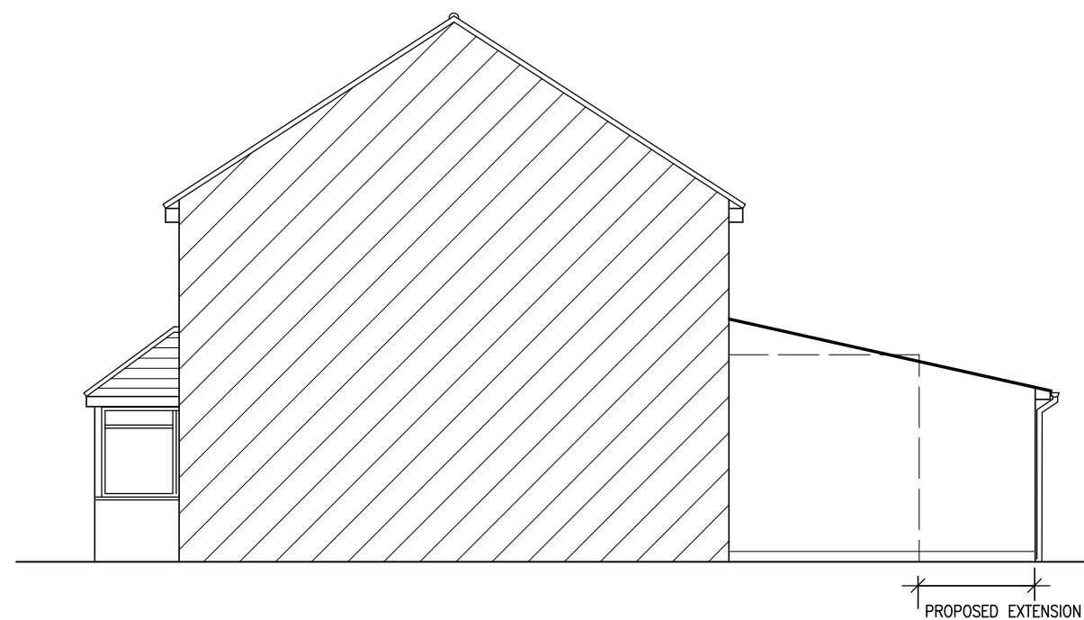
SIDE ELEVATION (THROUGH PARTY WALL)
