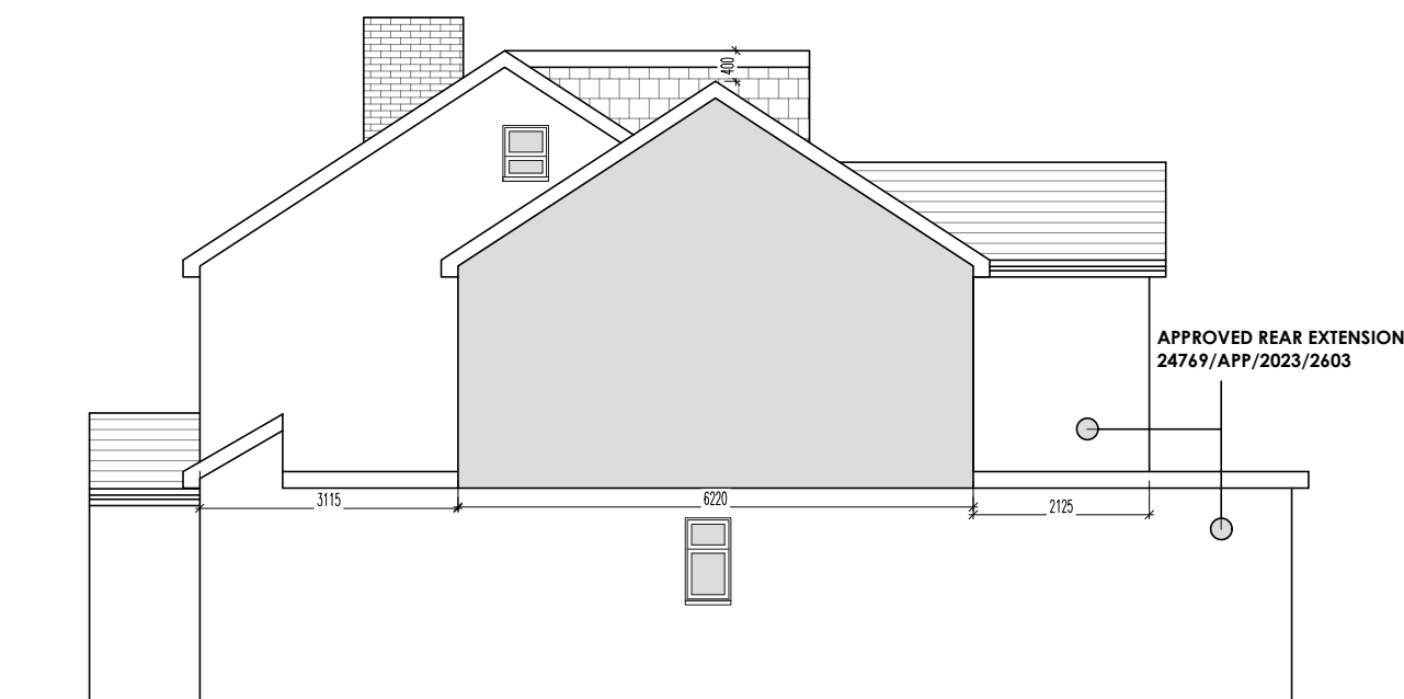
PROPOSED SIDE ELEVATION (FROM NO 17) SCALE 1/100
