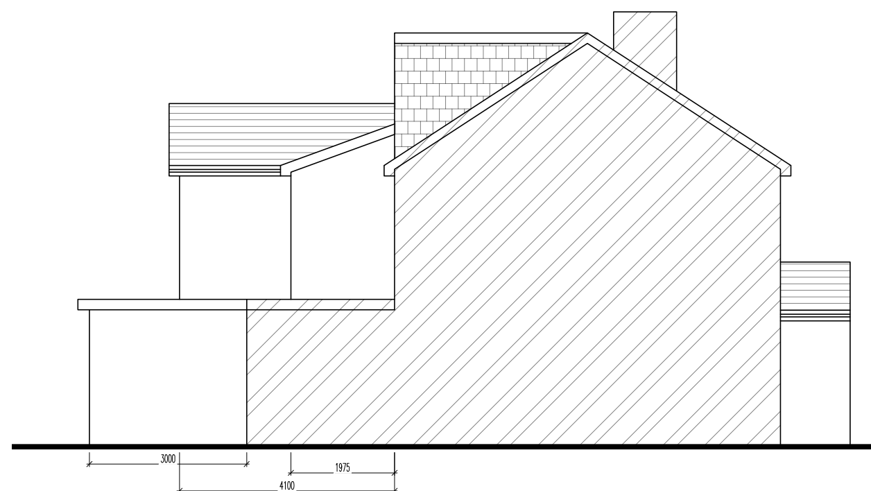
PROPOSED SIDE ELEVATION (FROM NO 13) SCALE 1/100
