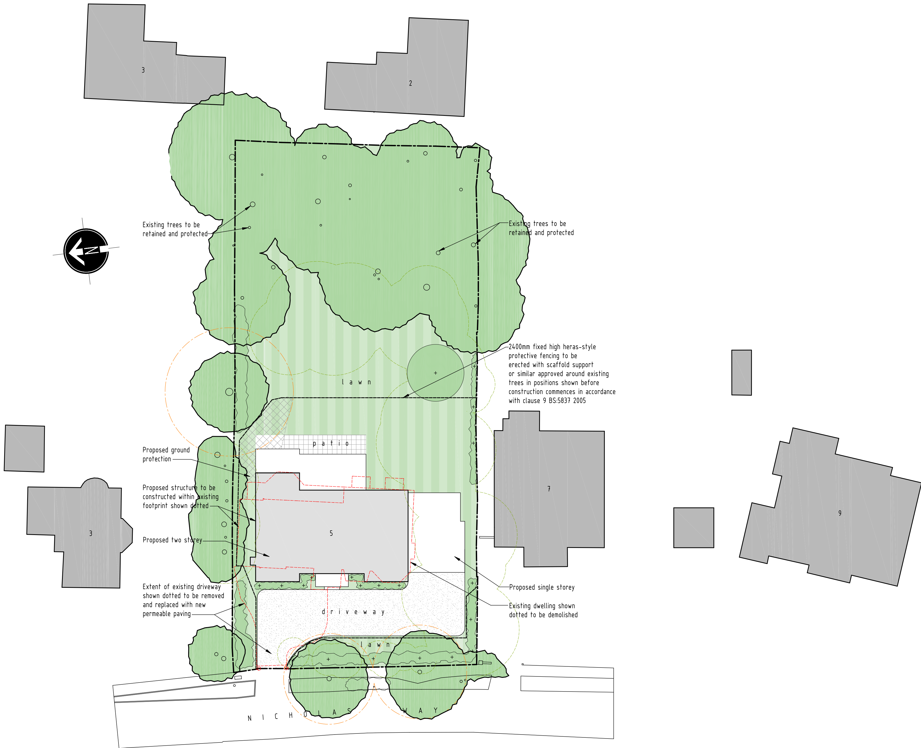
SITE LAYOUT PLAN - SCALE 1:250
