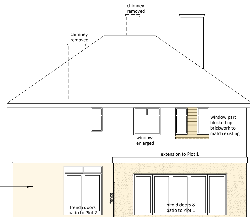
SOUTH-EAST ELEVATION
