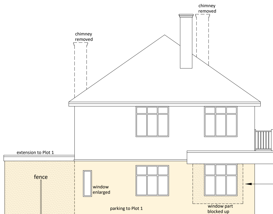
NORTH-EAST ELEVATION
