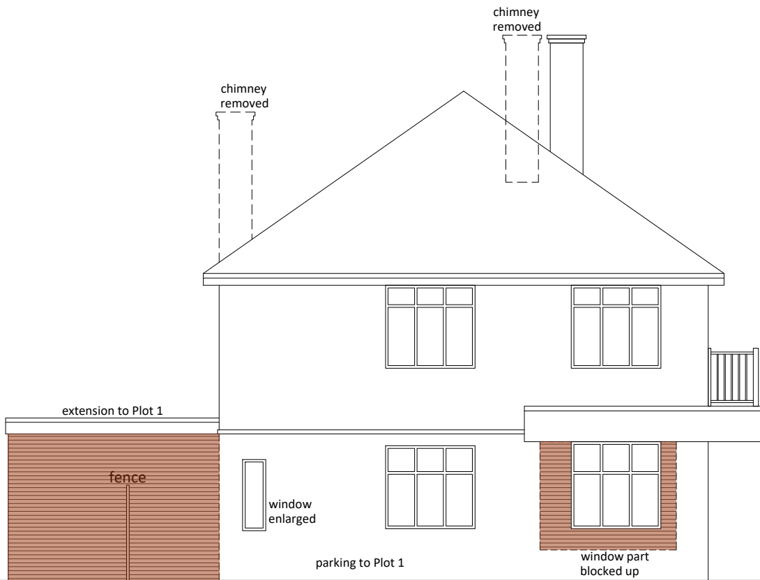
NORTH-EAST ELEVATION
