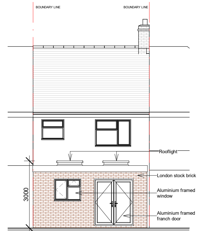
PP-PROPOSED REAR ELEVATION 1 : 100
