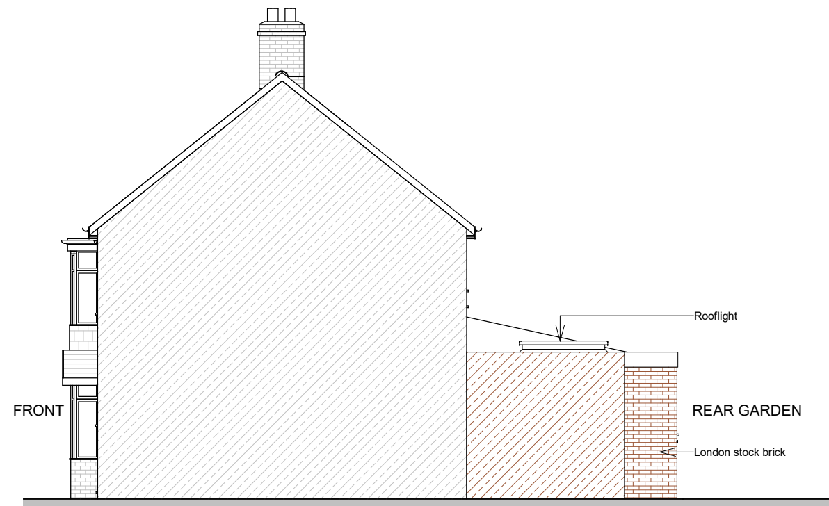
PP-PROPOSED EAST SIDE ELEVATION 1 : 100
