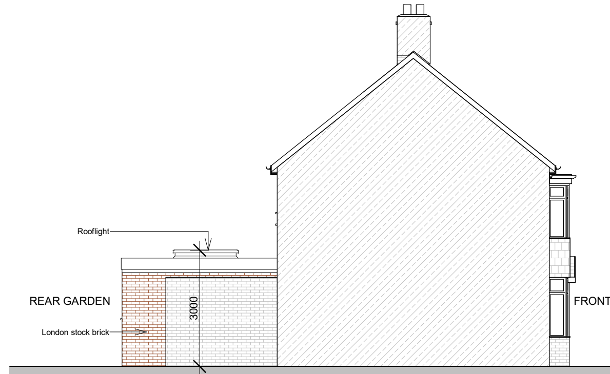
PP-PROPOSED WEST SIDE ELEVATION 1 : 100
