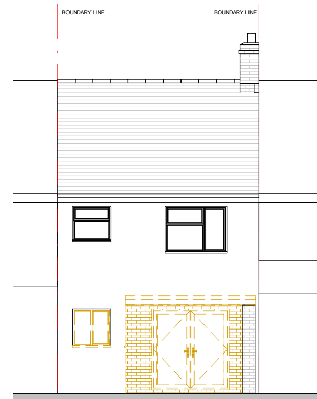
PP-EXISTING REAR ELEVATION 1 : 100
