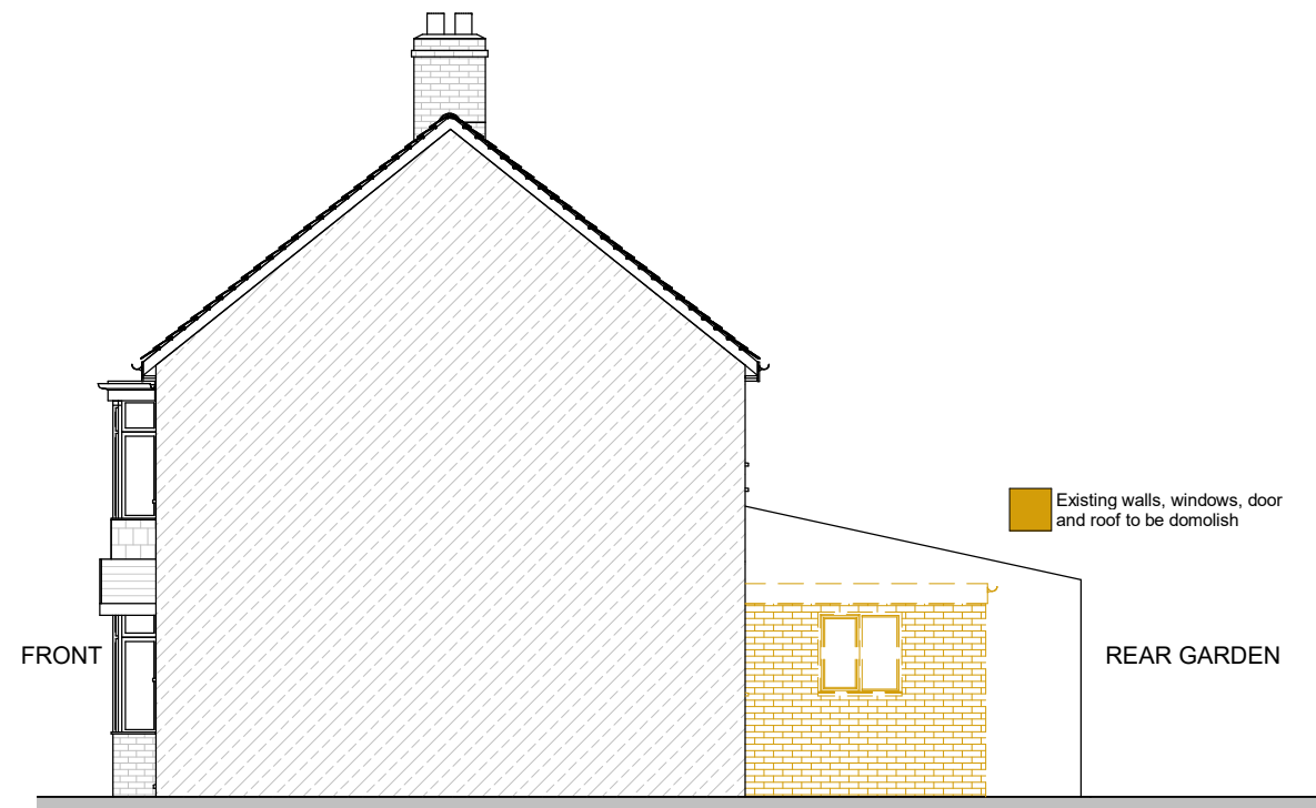
PP-EXISTING EAST SIDE ELEVATION 1 : 100
