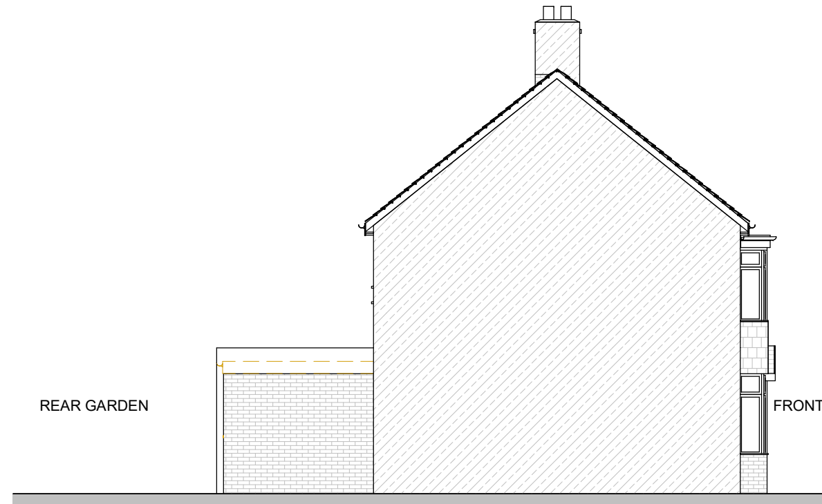
PP-EXISTING WEST SIDE ELEVATION 1 : 100
