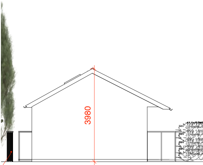
Side Elevation
