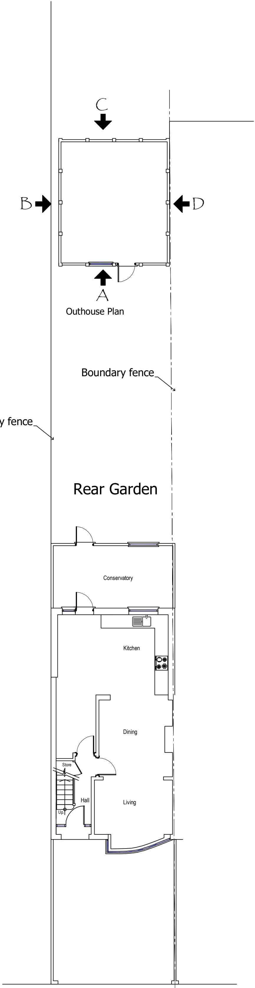
Existing Ground Floor Plan (scale: 1:100)
