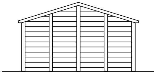
Existing Elevation 'C'
