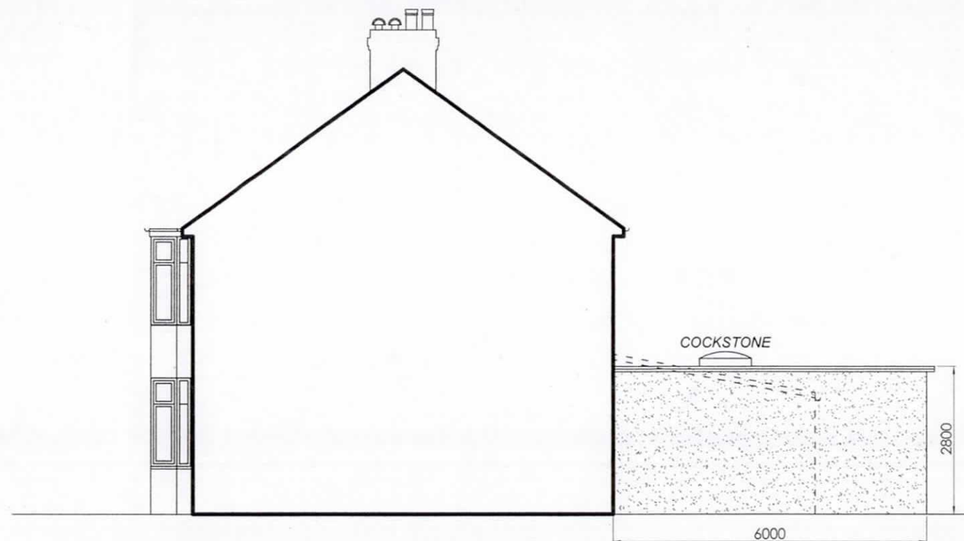
PROP SIDE ELEV 1/100
