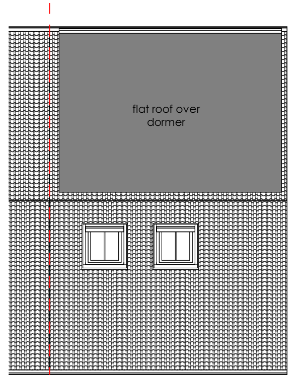
7 Proposed Roof Plan 2415-A-101 1 : 100
