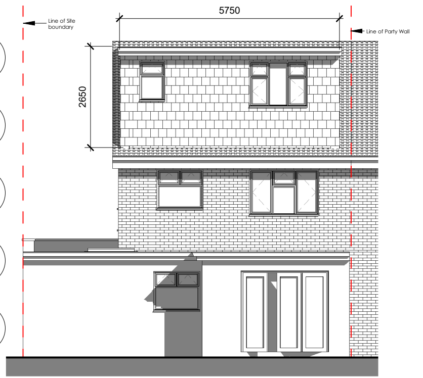
4 Proposed Rear Elevation 2415-A-101 1 : 100
