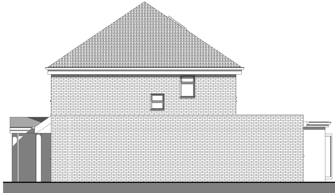
5 Existing Side Elevation 2415-A-100 1 : 100
