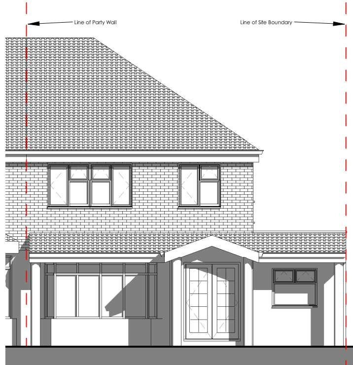
4 Existing Front Elevation 2415-A-100 1 : 100
