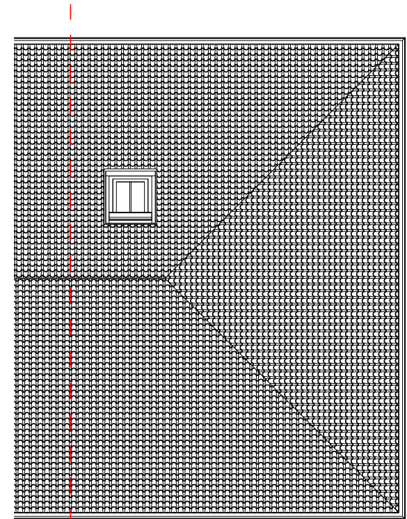
3 Existing Roof Plan 2415-A-100 1 : 100
