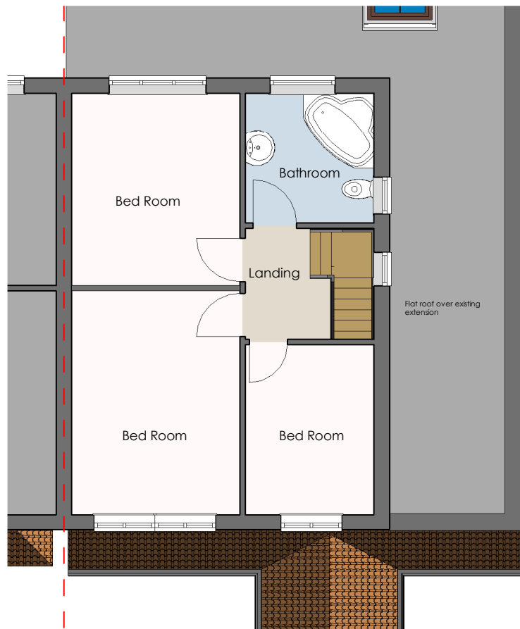
2 Existing First Floor 2415-A-100 1 : 100
