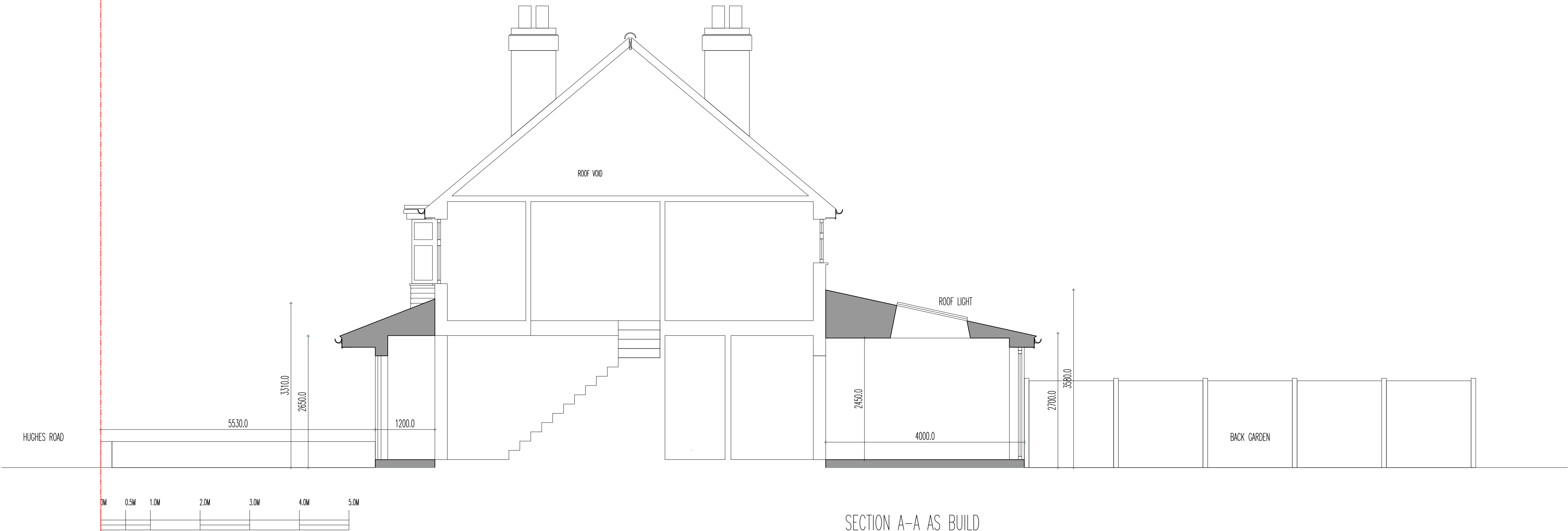
SECTION A-A AS BUILD
