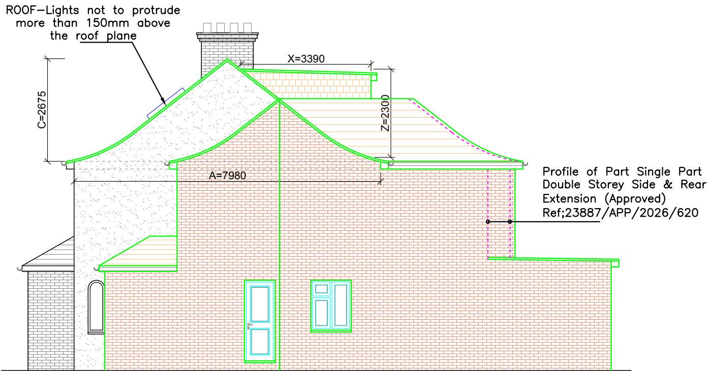
PROPOSED SIDE (P-No.16) ELEVATION SCALE= 1:100
