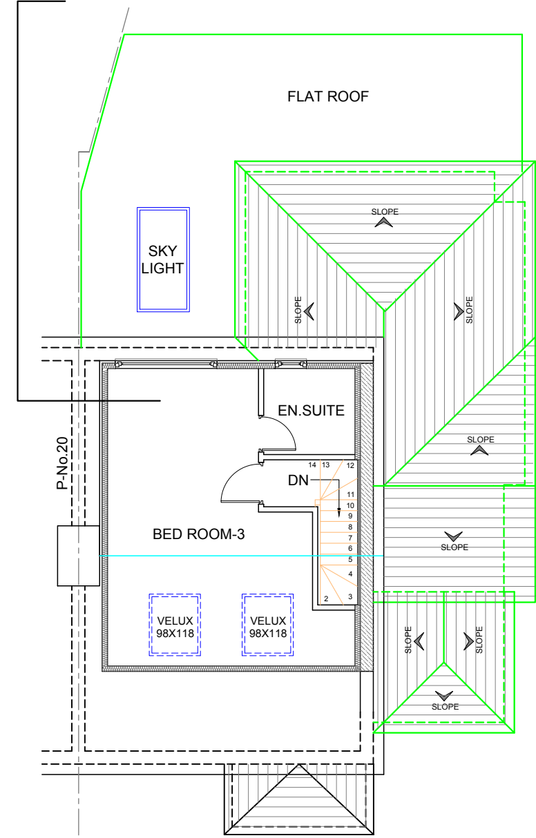
PROPOSED LOFT FLOOR PLAN SCALE= 1:100
