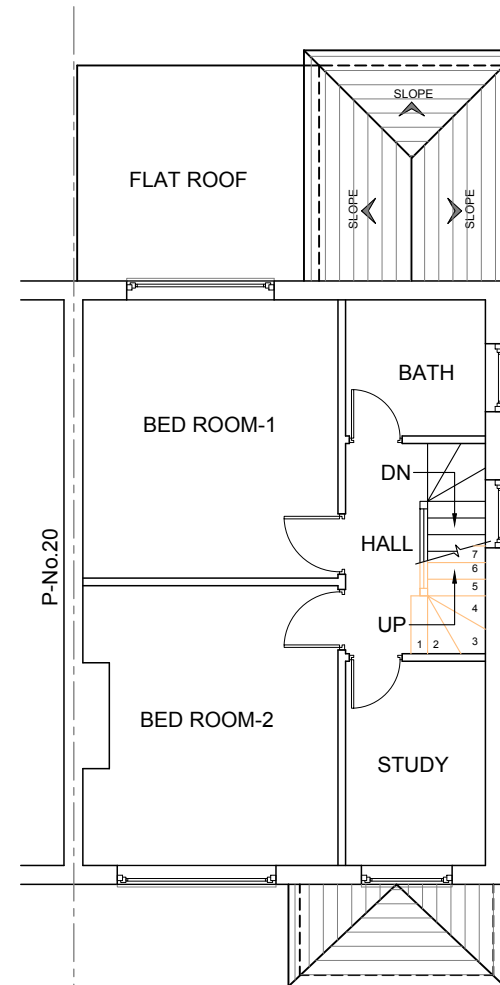
PROPOSED FIRST FLOOR PLAN SCALE= 1:100
