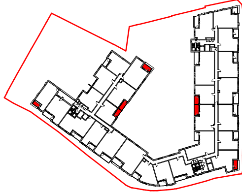
4 Privacy Screen Location - Level 3
