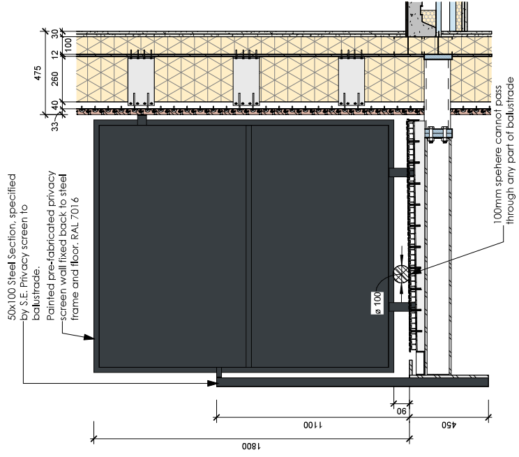
2 Corner Balcony Privacy Screen - Elevation
