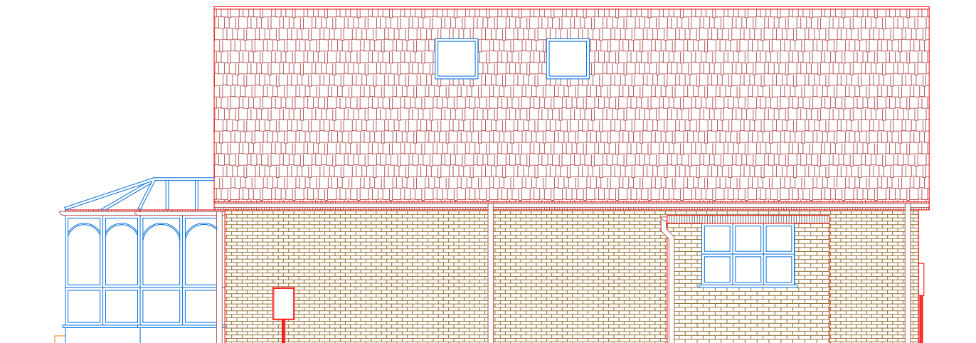
EXISTING SIDE ELEVATION-1
