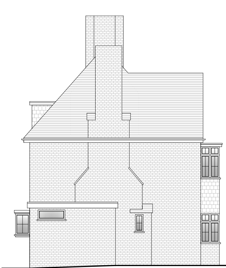
6 Existing Side Elevation
