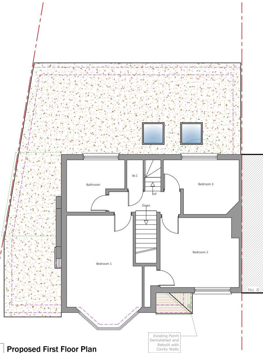
2 Proposed First Floor Plan
