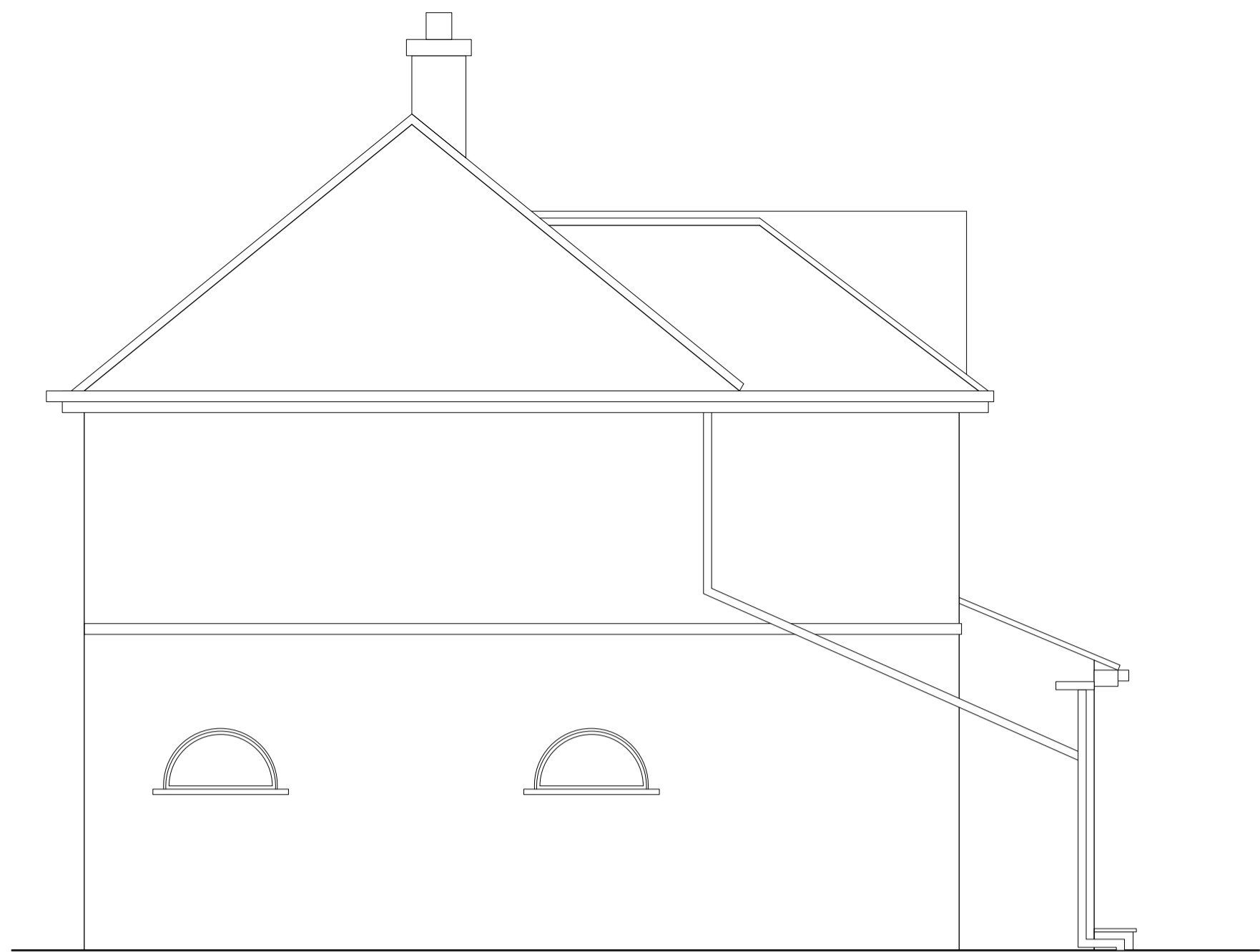
1 EAST Scale 1:50
