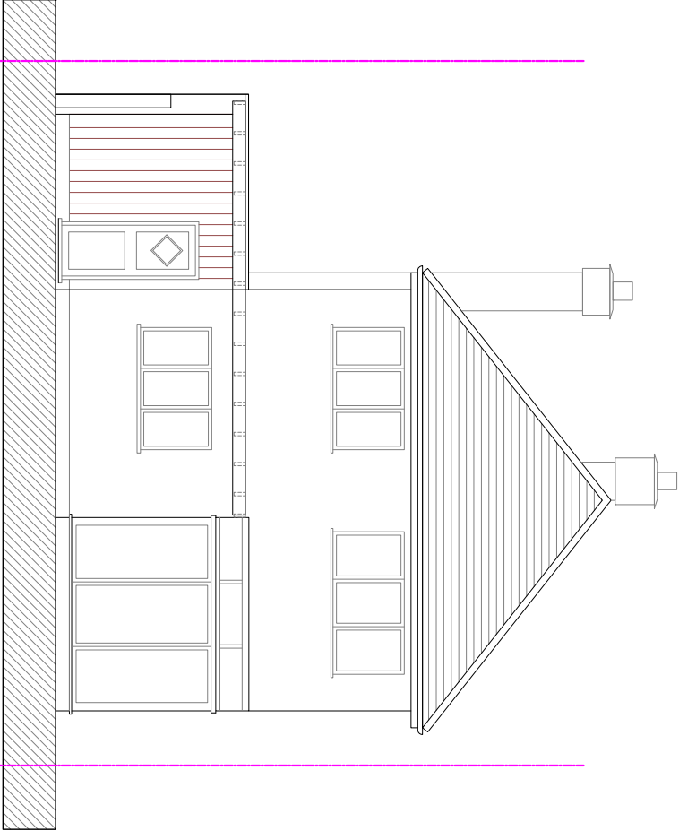
3 REAR ELEVATION
