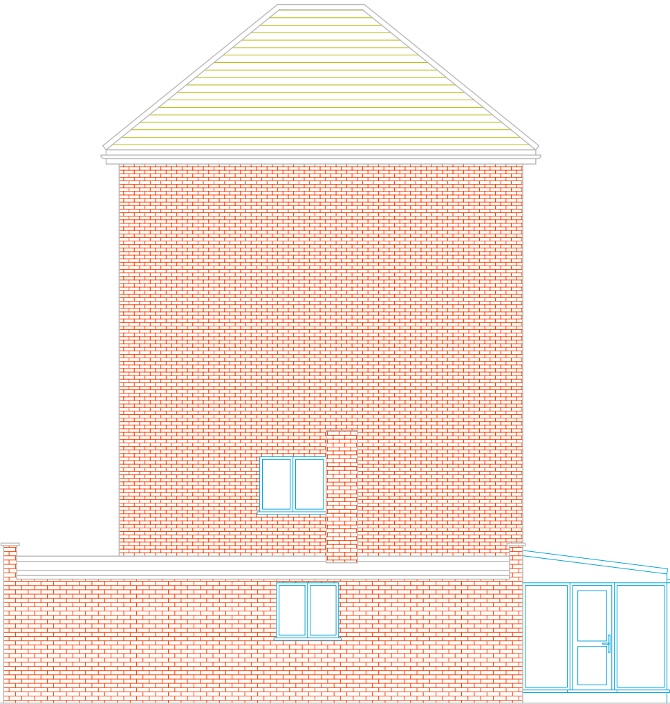
PROPOSED SIDE ELEVATION-1
