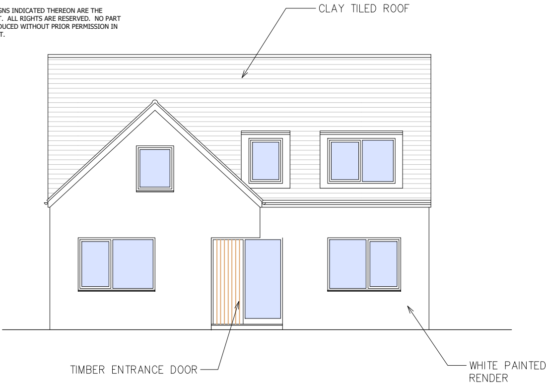
1 PROPOSED NORTH ELEVATION 1 : 100
