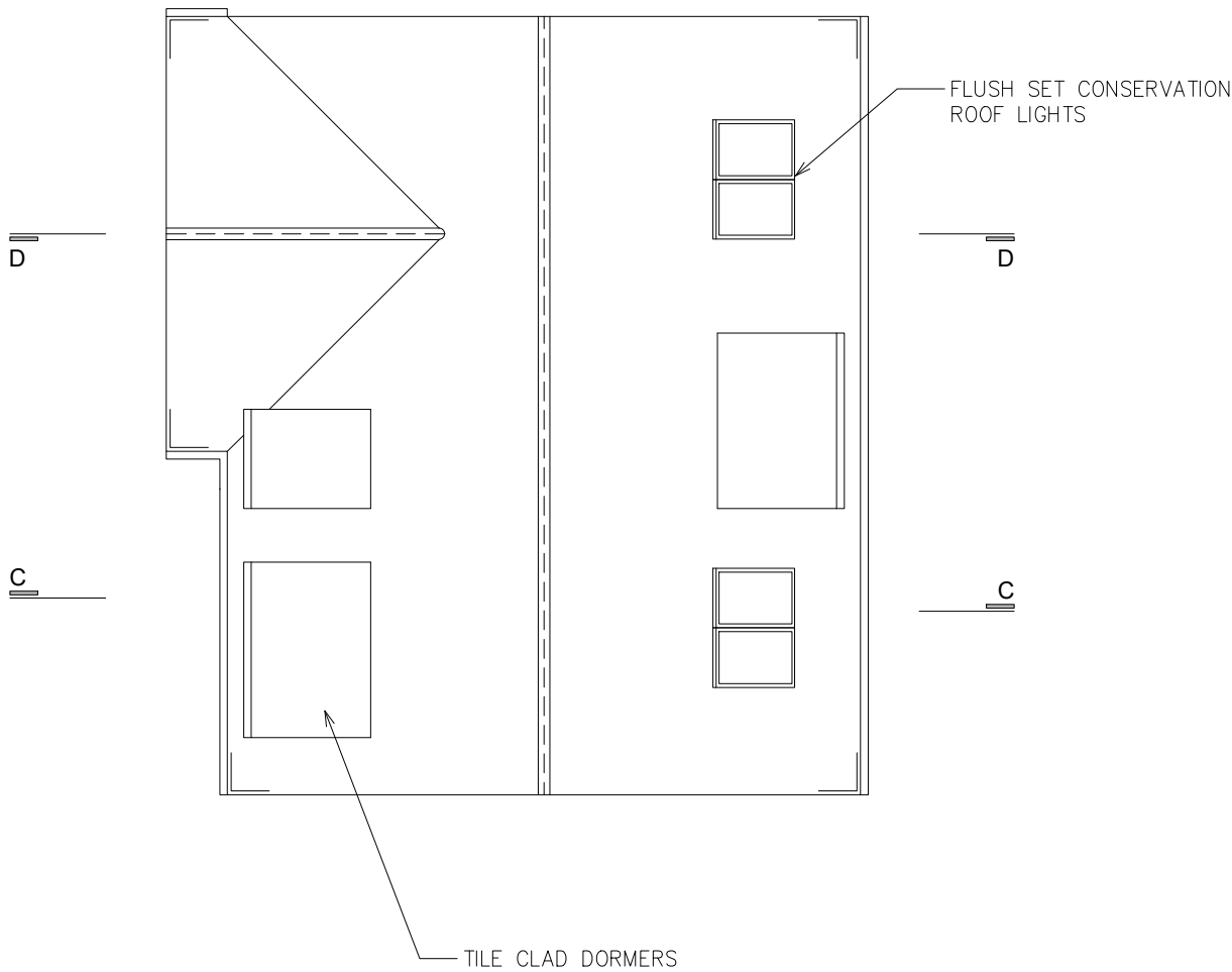
1 PROPOSED ROOF PLAN 1 : 100
