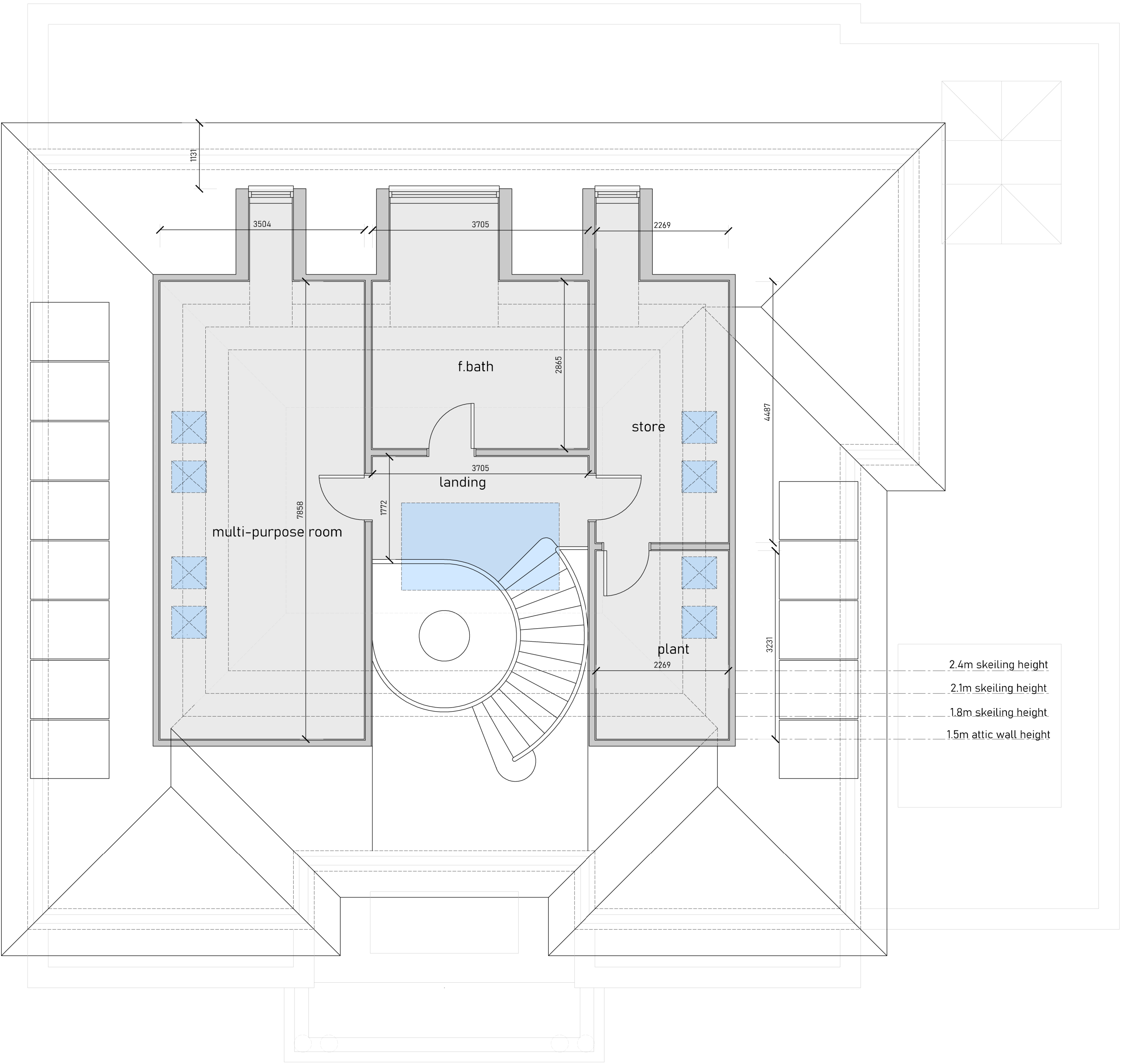
ROOF AREA PLAN SCALE 1:50
