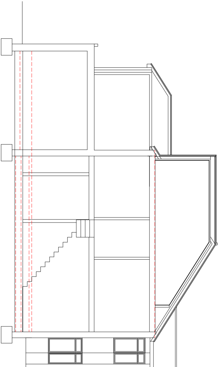
SECTION A
