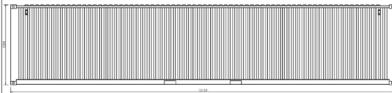
40ft Shipping Container - Side Elevation
