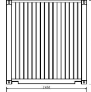
40ft Shipping Container - Door Elevation
