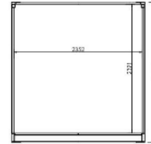
40ft Shipping Container - Section
