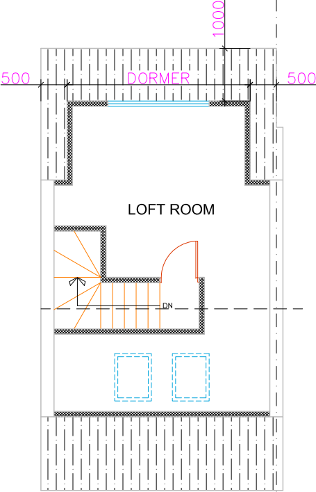
PROPOSED LOFT PLAN
