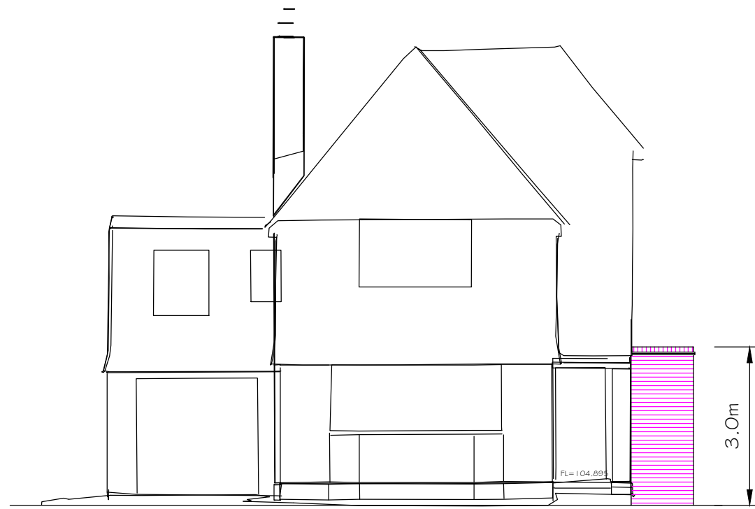
FRONT ELEVATION (SOUTH EAST)
