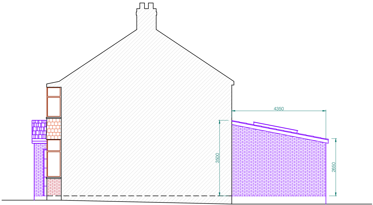
South-east elevation
