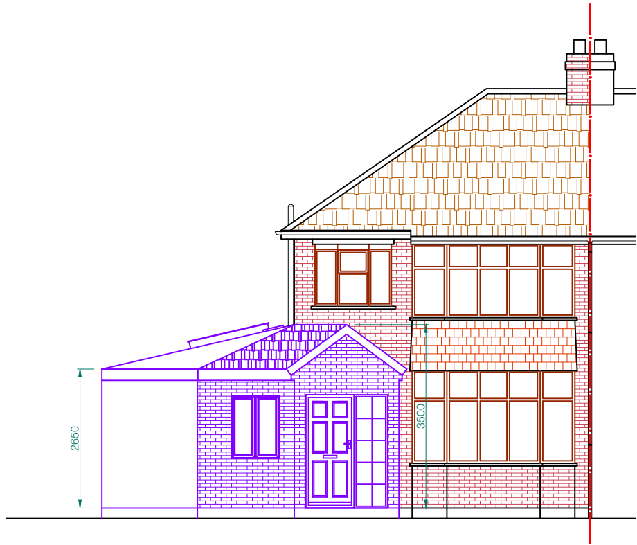
South-west elevation
