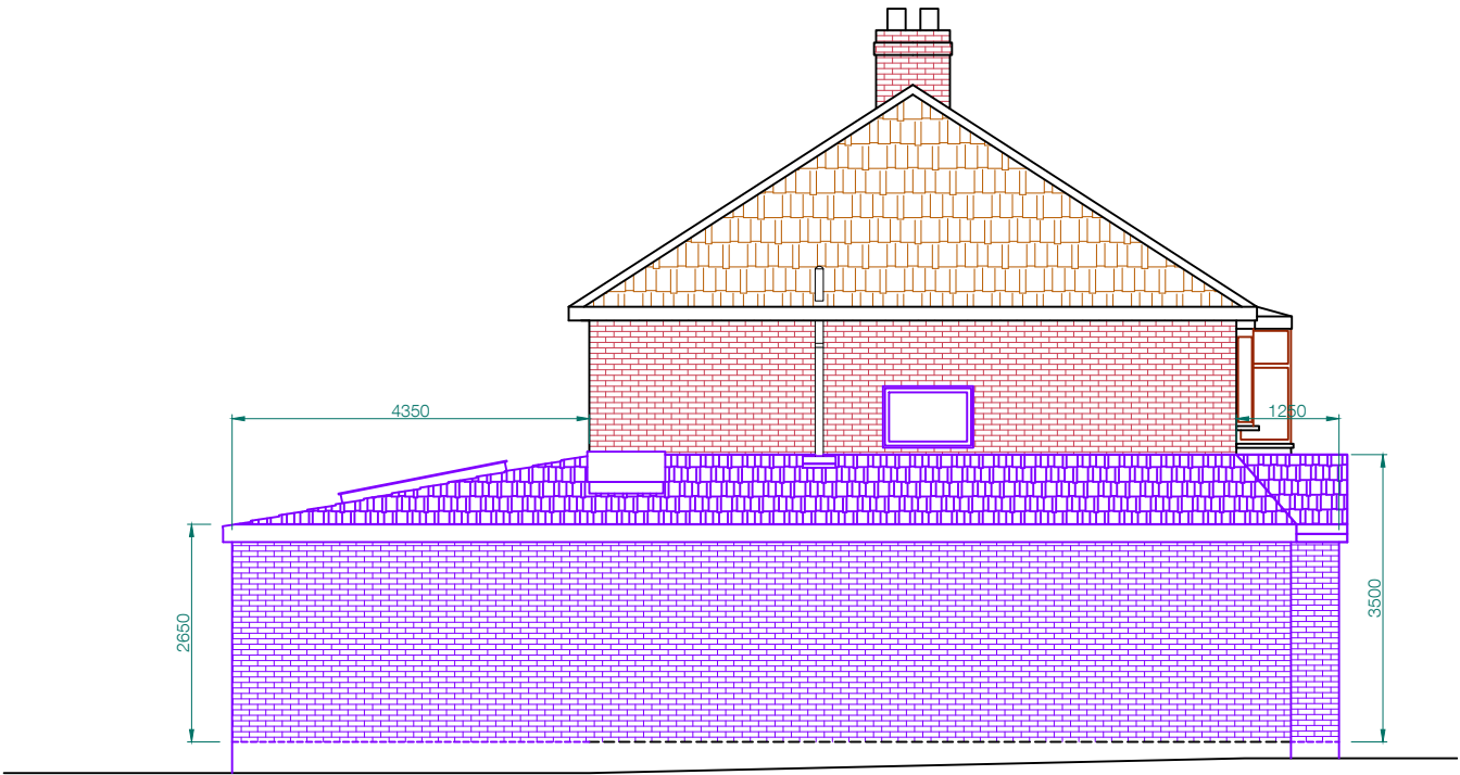
North-west elevation
