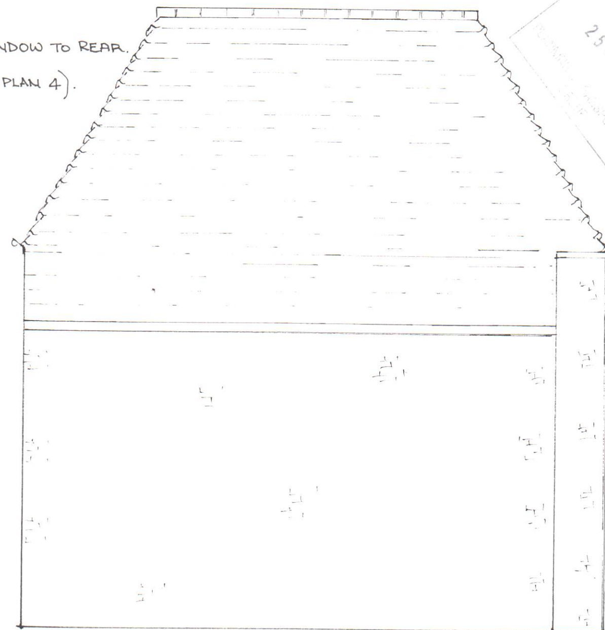
West elevation 1:50 PROPOSED
