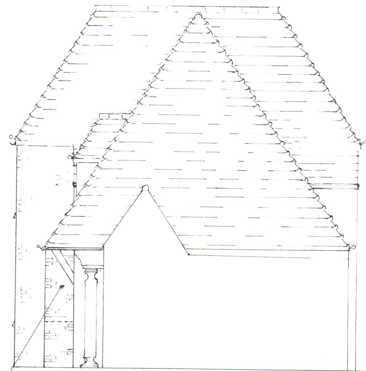
East elevation 1:50 PROPOSED
