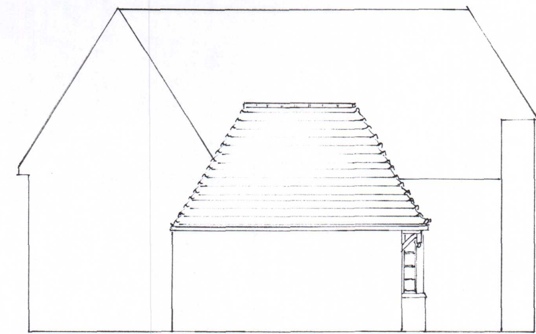
west elevation 1:100
