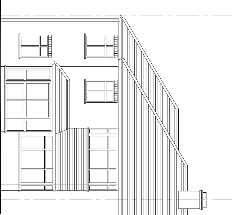
PRE EXISTING FRONT ELEVATION
