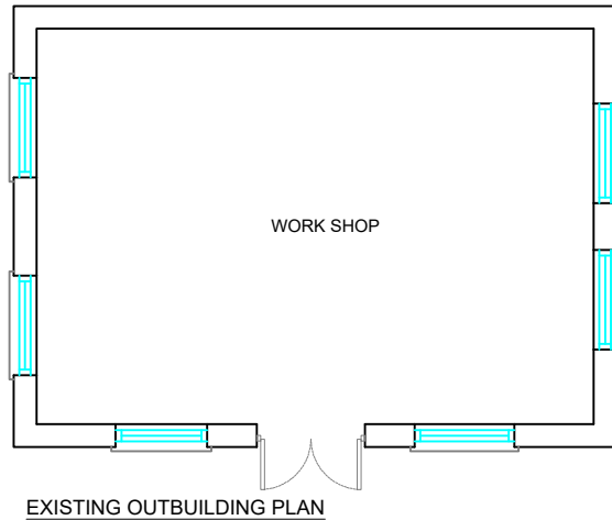
EXISTING OUTBUILDING PLAN
