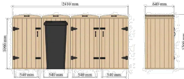
Bellus Quad Wheelie Bin Storage For 140 Litre Bin Dimensions:
