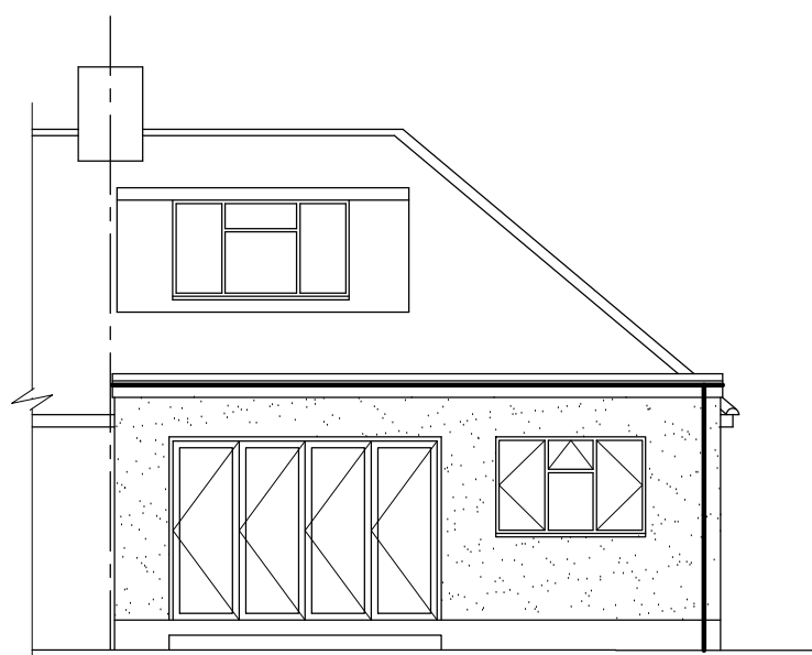
REAR ELEVATION (1:100)
