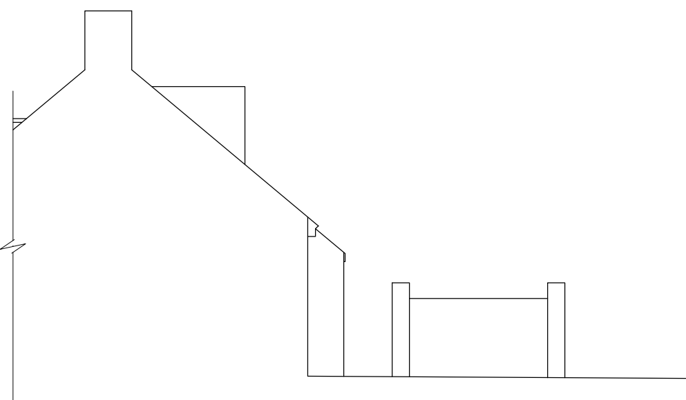
RIGHT ELEVATION (1:100)
