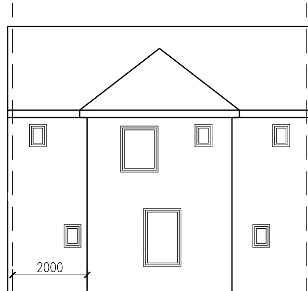
Proposed Rear
