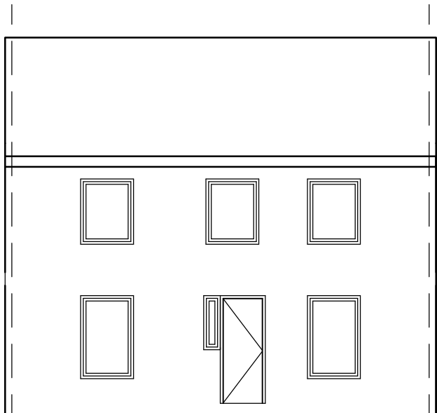
Proposed Front
