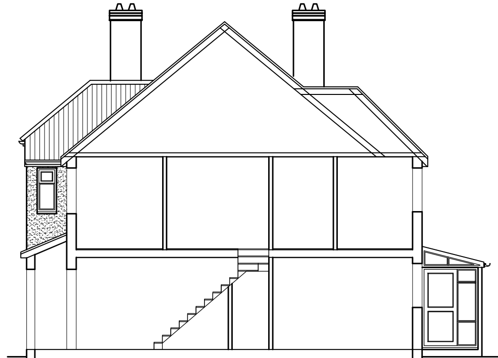
EXISTING SECTION
