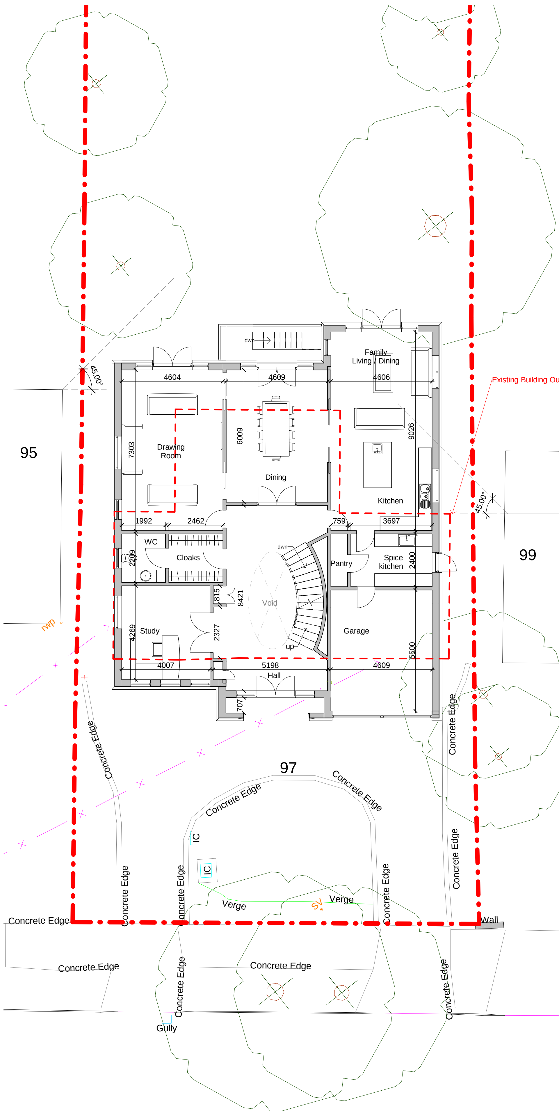
1 01.Ground Floor 1 : 100
