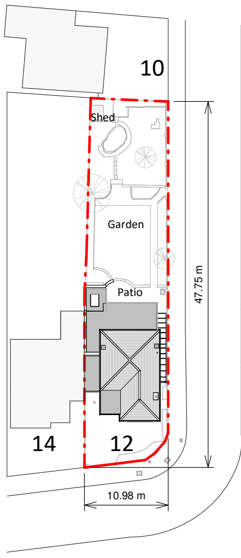
Block Plan
