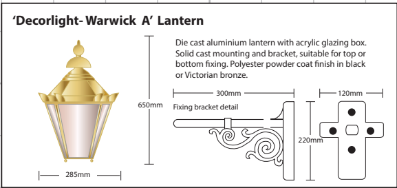
G TWO X NEW LANTERNS SIZE. 0.28m x 650mm. H.A.G. 2.5m.
