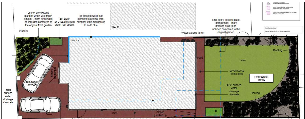
Figure 10: Proposed Site Plan (Please refer to full drawing for annotations)
