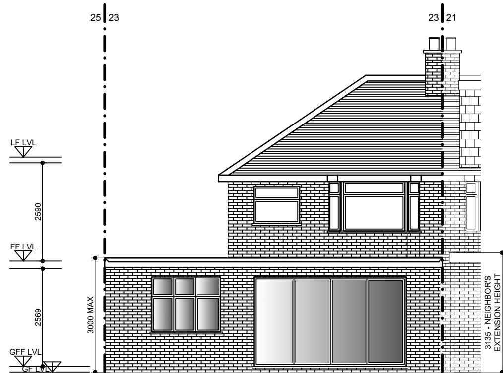
REAR ELEVATION PROPOSED
