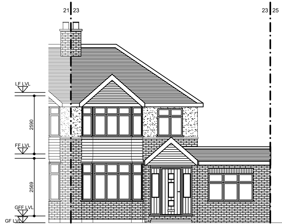
FRONT ELEVATION PROPOSED - NO CHANGE
