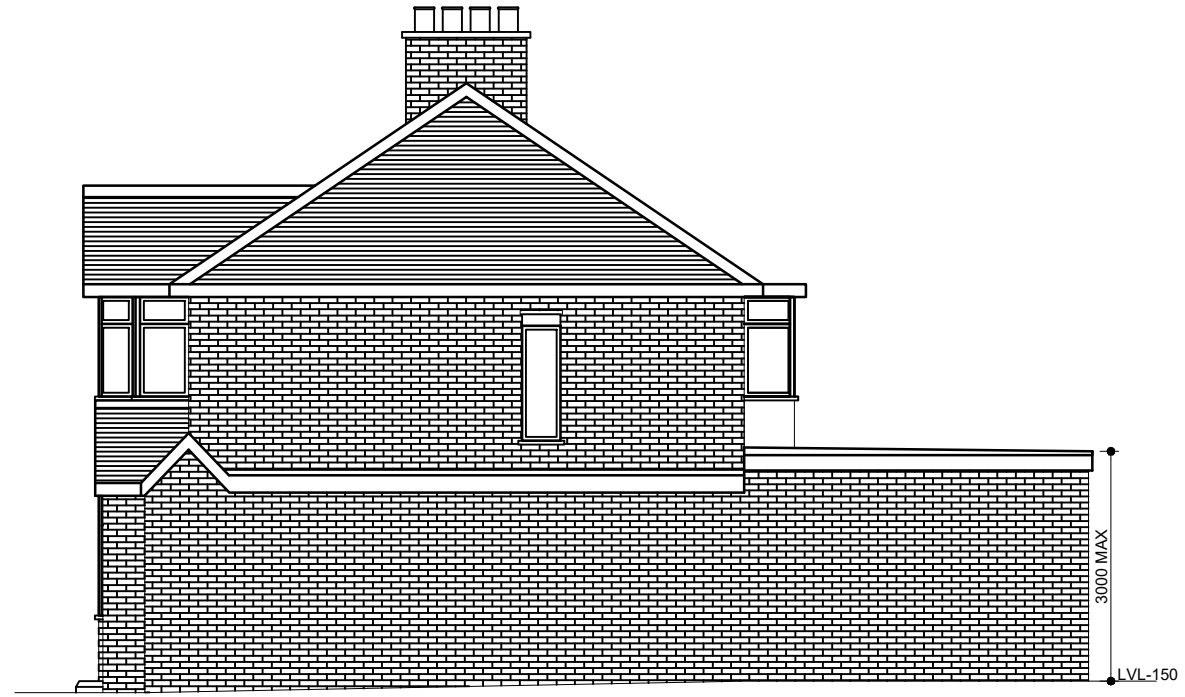
SIDE ELEVATION PROPOSED (AS VIEWED FROM NO:25)
