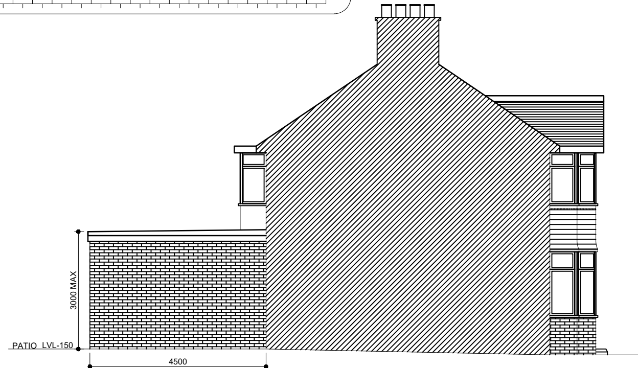
SIDE ELEVATION PROPOSED (AS VIEWED FROM NO:21)
